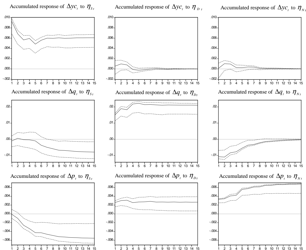
Figure 7. Impulse-response functions
