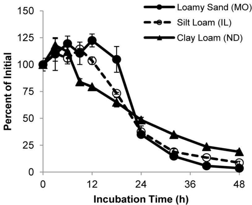
Figure 4: Degradation of DvSnf7 RNA degradation in three soil samples (Dubelman et al, 2014): DvSnf7 RNA was added (7.5 \mu\text{g} per gram of soil) in the absence of maize tissue, then its concentration determined after different incubation times with a QuantiGene assay. Error bars represent one standard error of the mean ( n = 2 ). Soil samples were from Missouri (MO), Illinois (IL), and North Dakota (ND). [Equivalent results were obtained from soil samples amended with lyophilised insect-protected maize tissue and fortified with 7.5 mg DvSnf7 RNA per gram of soil.]
