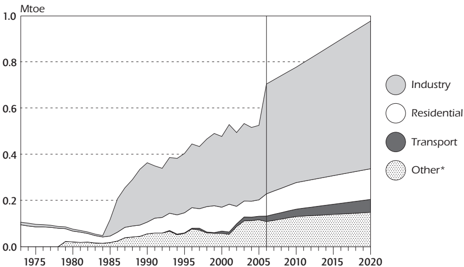
Final Consumption of Natural Gas by Sector, 1973 to 2020
