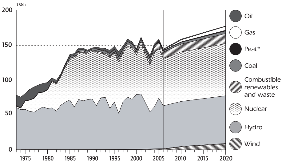
Figure 17 Electricity Generation by Source, 1973 to 2020
