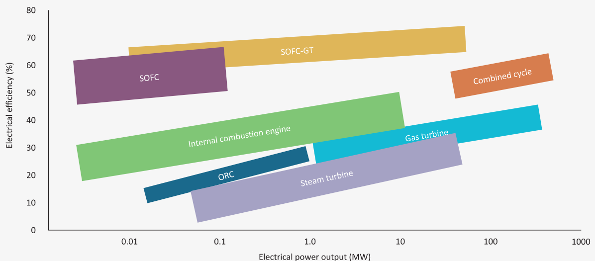
Figure 7.10. Generation efficiency and scale
