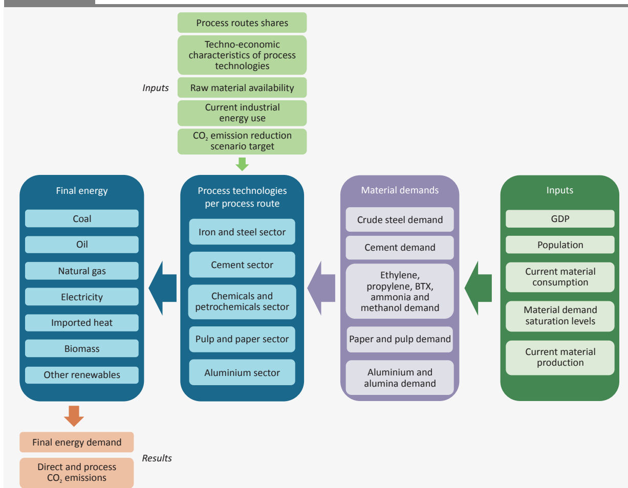
Figure A.4. Structure of ETP industry model
