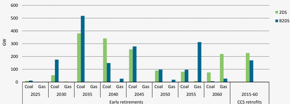
6.25. Early retirements and CCS retrofits of coal- and gas-fired capacity in the 2DS and B2DS
