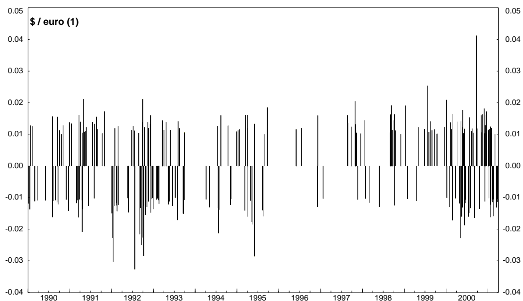
Figure 3. High-frequency exchange rate volatility (daily changes exceeding 1 percentage point)
